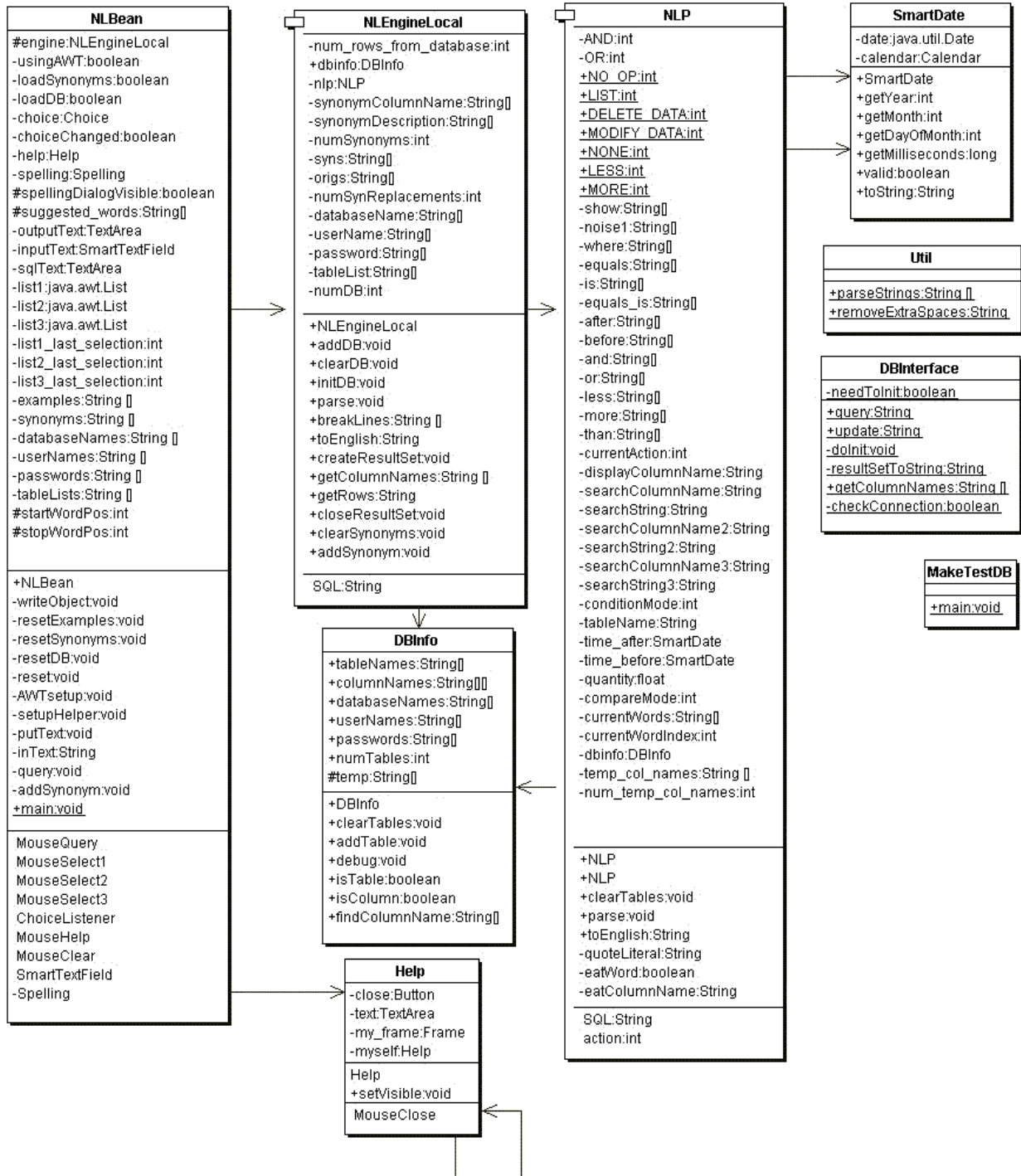
Figure 2.4 UML class diagram for the NLBean system
