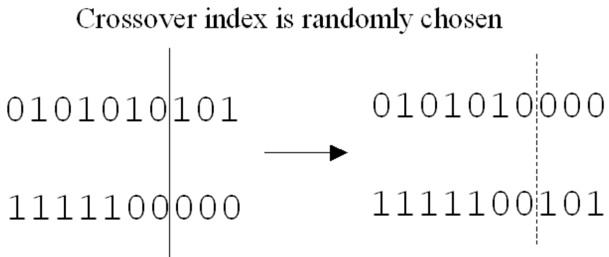
Figure 4.2 Crossover operation
