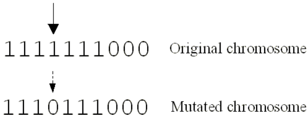
Figure 4.3 Mutation operation
